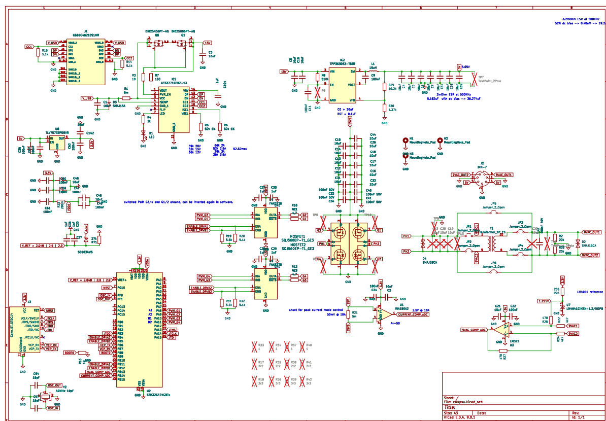
Figure 1: Schematic SVG
